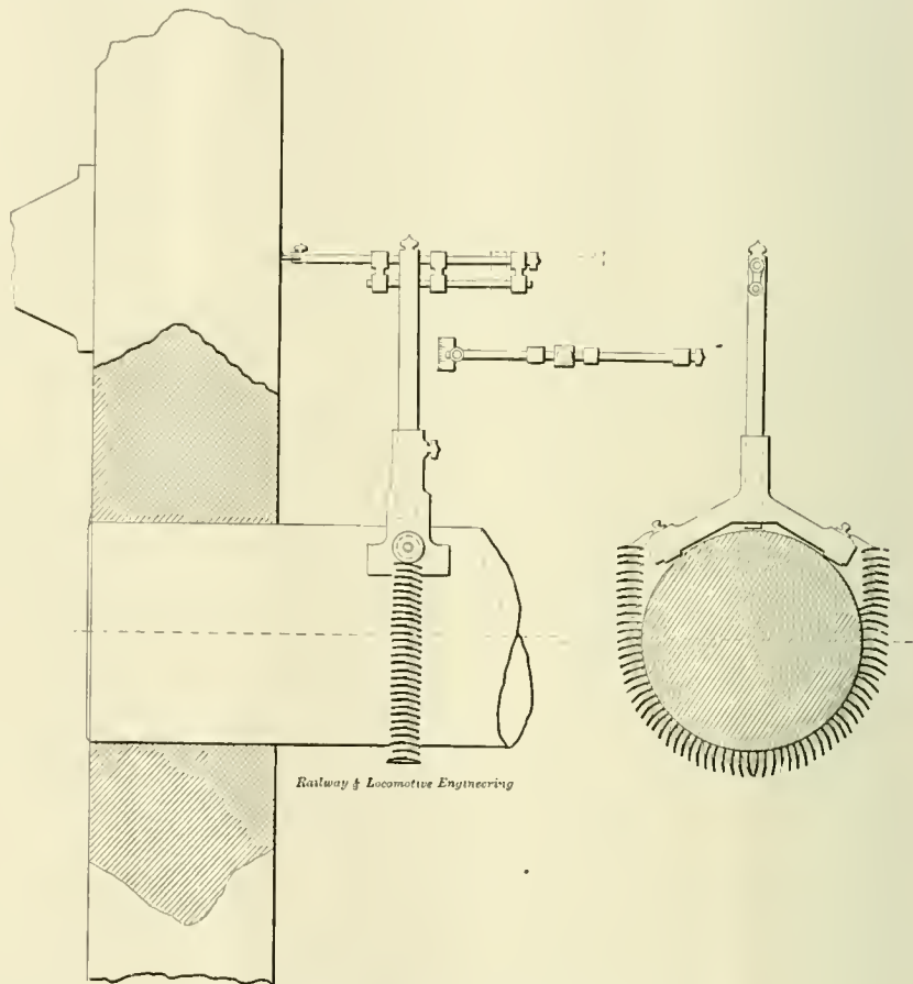
GAUGE FOR TWISTING WHEEL CENTERS.
